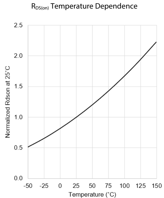
Figure 12: Normalized R_{DS(on)} as a function of T_J
