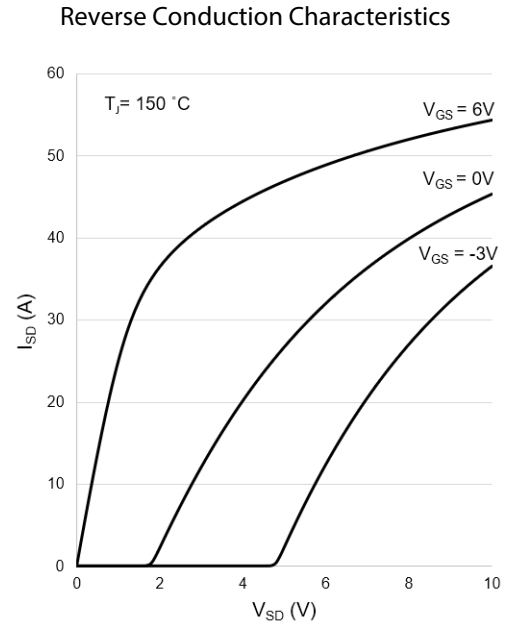
Figure 10: Typical I_{SD} vs. V_{SD} at 150 °C
