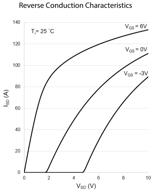
Figure 9: Typical I_{SD} vs. V_{SD} at 25 °C
