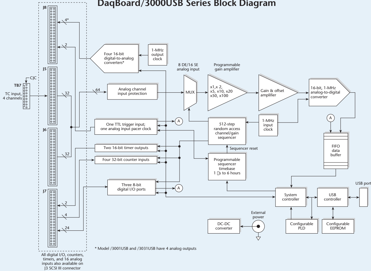
DaqBoard/3000USB Series Block Diagram
