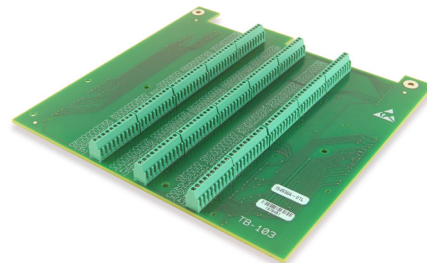
TB-103 termination board mounts directly onto a USB-2600 Series board
