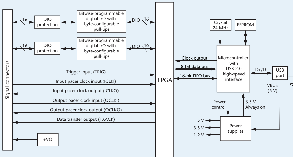
USB-DIO32HS Block Diagram
