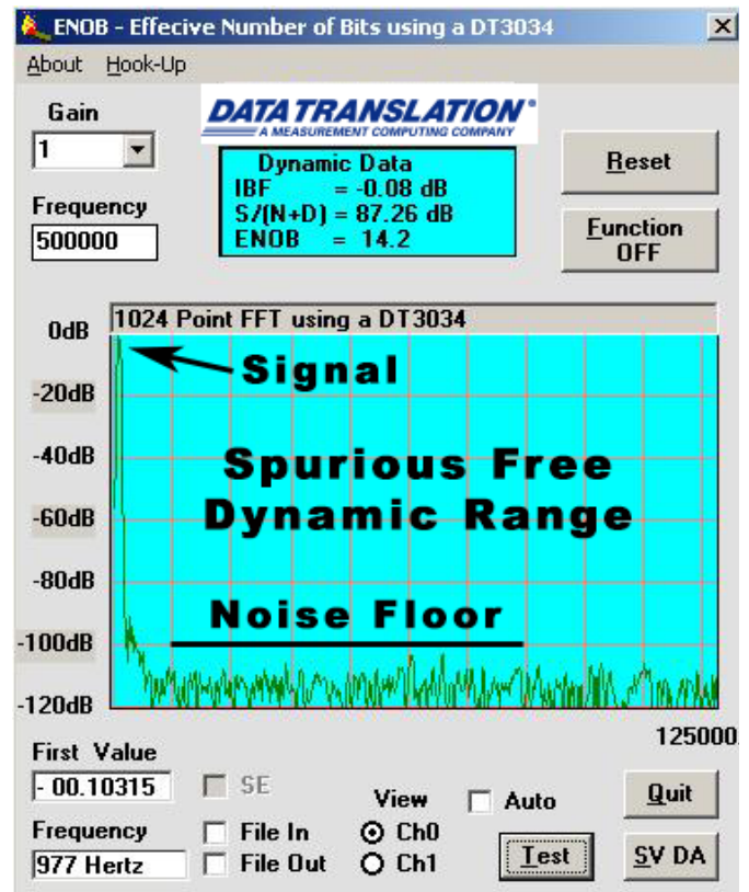
The DT3034 is a high-speed, high-resolution data acquisition board for the PCI Bus.
