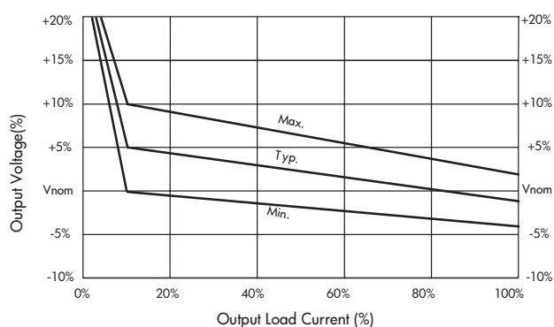
Graph 1: Load regulation
