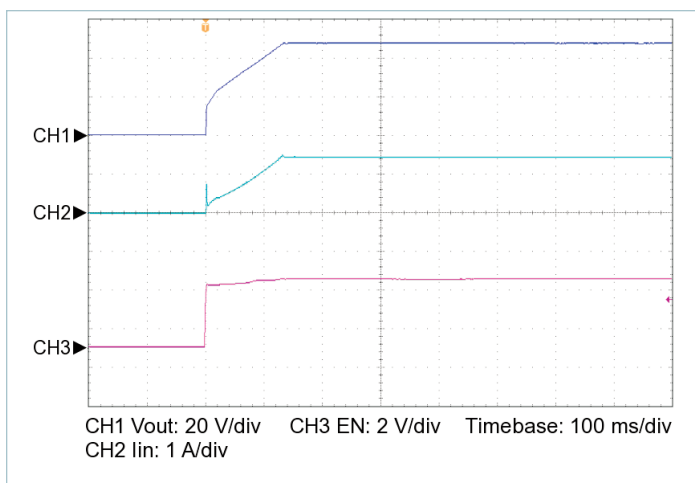
Figure 17 — Startup from EN, V_{IN} = 275\text{ V} , C_{OUT\_EXT} = 2000\text{ μF} , R_{LOAD} = 6.076\text{ Ω}
