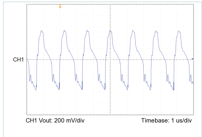
Figure 19 — Output voltage ripple, V_{IN} = 275\text{ V} , V_{OUT} = 48.0\text{ V} , C_{OUT\_EXT} = 200\text{ μF} , R_{LOAD} = 6.076\text{ Ω}
