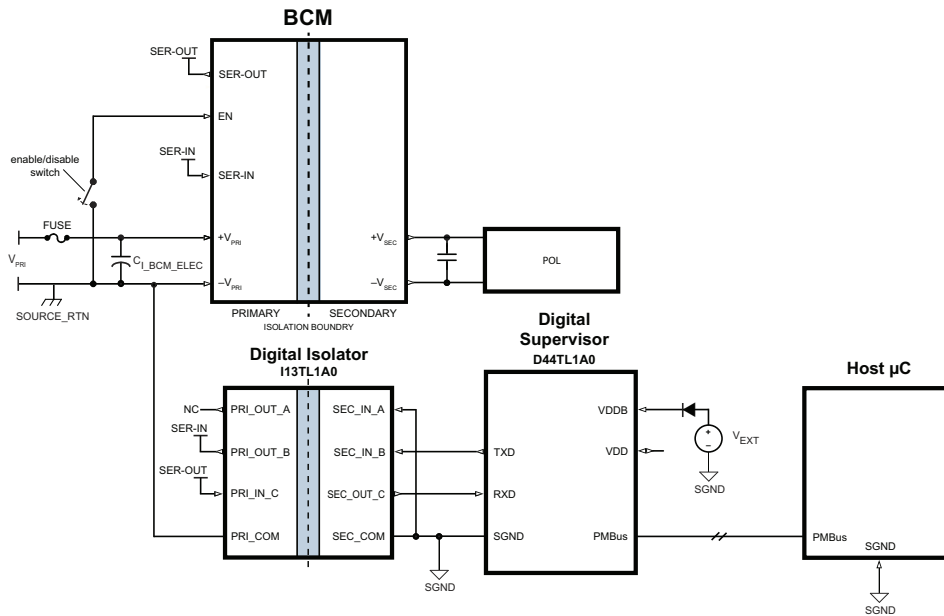
BCM6123xD1E13A2y01 at Point of load
