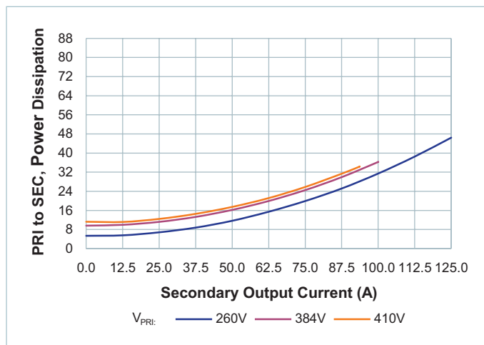
Figure 11 — Power dissipation at T_{CASE} = 90^{\circ}C
