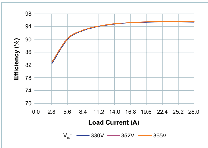
Figure 7 — Efficiency at T_{CASE} = 25^{\circ}\text{C}
