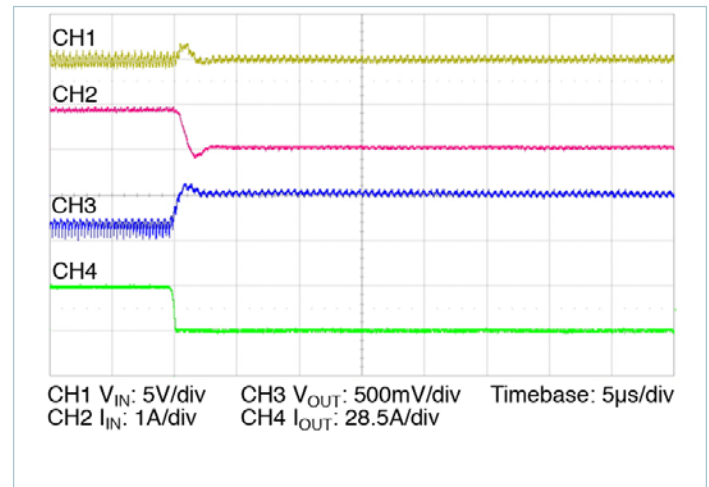
Figure 16 — 28.5A – 0A transient response: C_{IN} = 2.2\mu F , I_{IN} measured prior to C_{IN} , no external C_{OUT}
