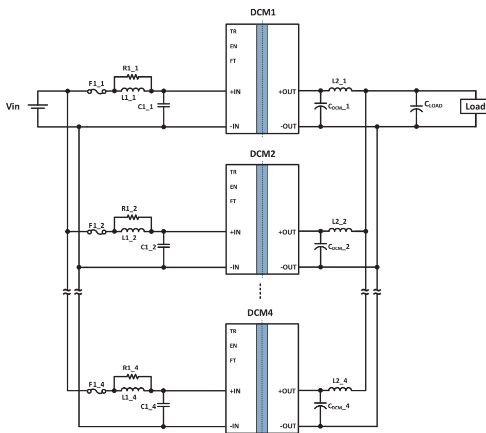
Typical Application 1: DCM48AP050x160A50 in an array of four units
