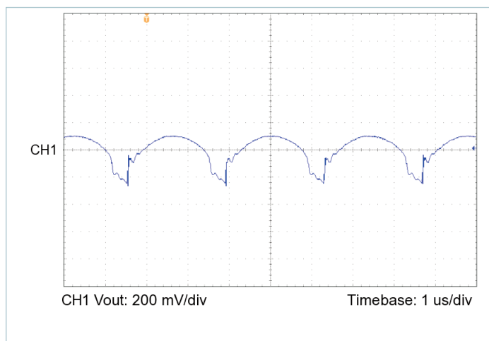
Figure 19 — Output voltage ripple, V_{IN} = 48\text{ V} , V_{OUT} = 5.0\text{ V} , C_{OUT\_EXT} = 1000\text{ }\mu\text{F} , R_{LOAD} = 0.156\text{ }\Omega
