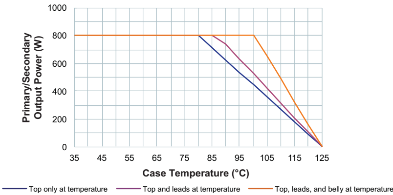
Figure 1 — Specified thermal operating area
