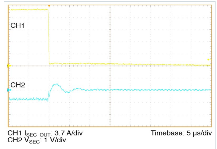
Figure 13 — 16.9 A – 0 A transient response: C_{PRI\_IN\_EXT} = 270 \mu F , no external C_{SEC\_OUT\_EXT}
