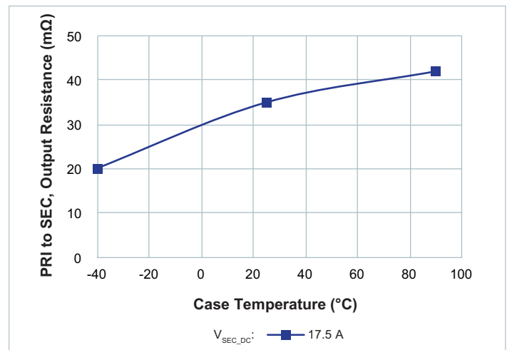
Figure 9 — R_{SEC} vs. temperature; Nominal V_{PRI\_DC} I_{SEC\_DC} = 17.5\text{ A} at T_{CASE} = 90^{\circ}\text{C}
