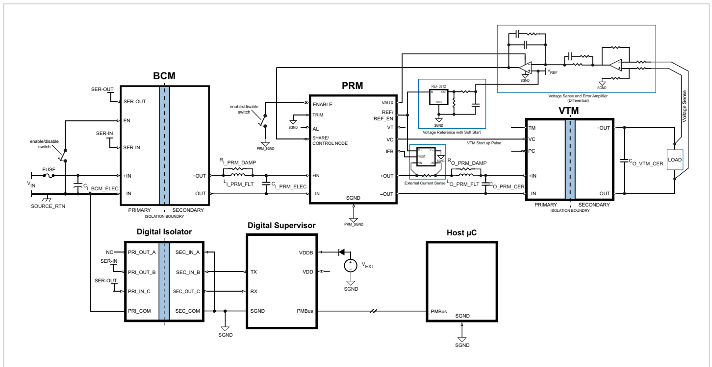
BCM380y475x1K2A31 + PRM + VTM, Remote Sense Configuration
