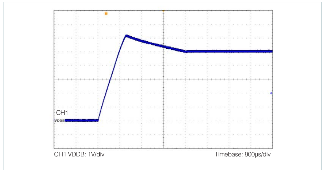
Figure 3 I2C-ADAPTER-A02 VDDB overshoot ( 6.2V_{PEAK} )
