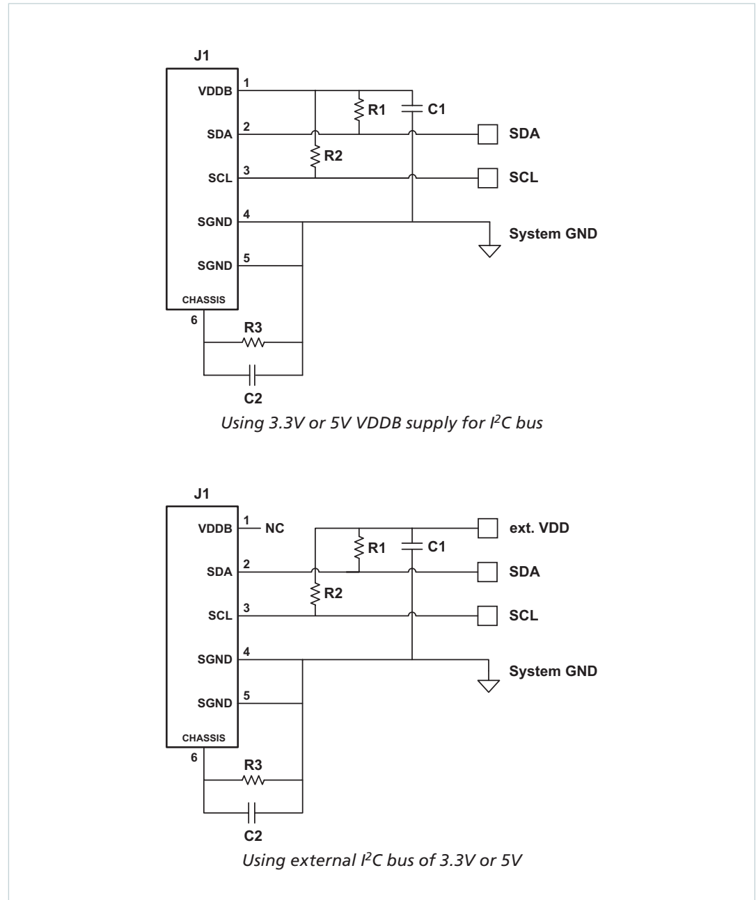
Figure 2 Recommended pull-up resistor configurations
