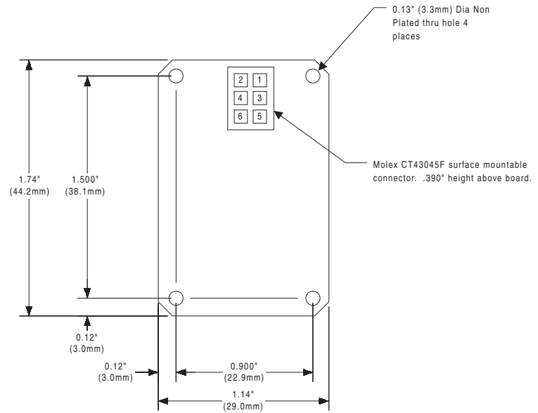
Figure 11. Mechanical Drawing
