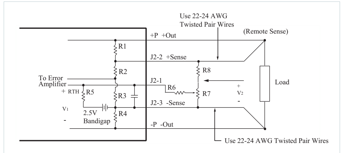
Figure 10. External Trim
