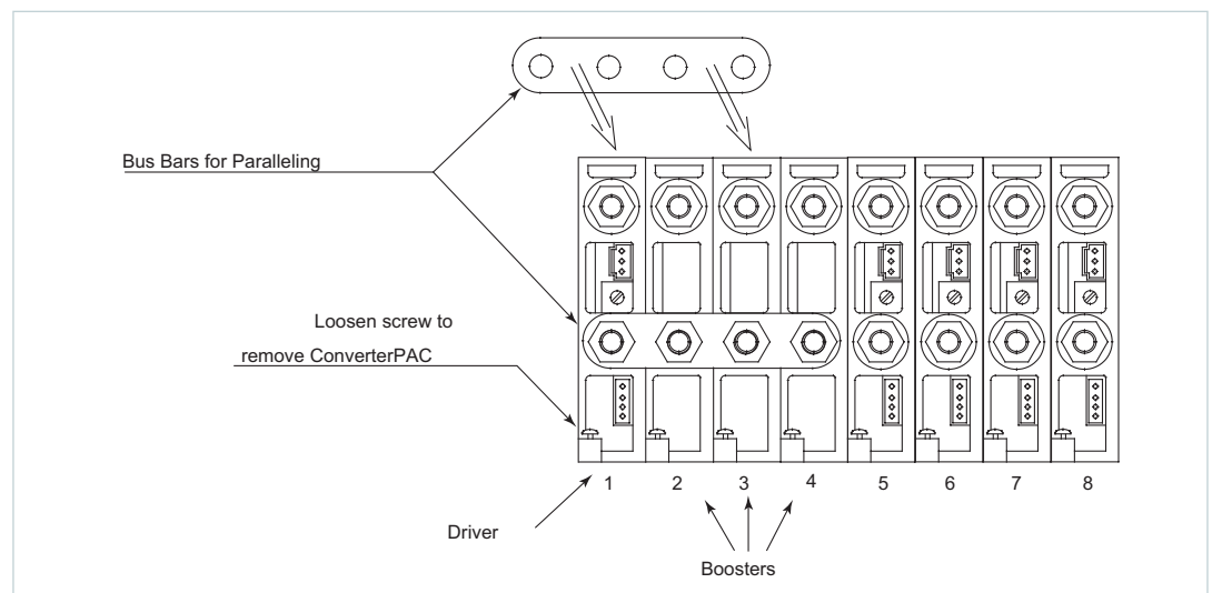
Figure 2. Paralleling ConverterPACs
