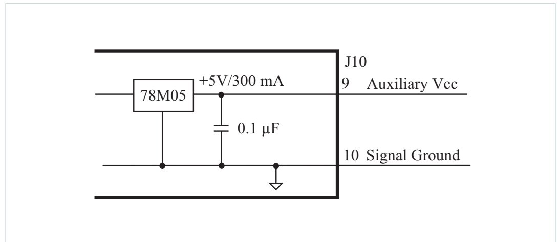
Figure 7. Auxiliary Vcc
