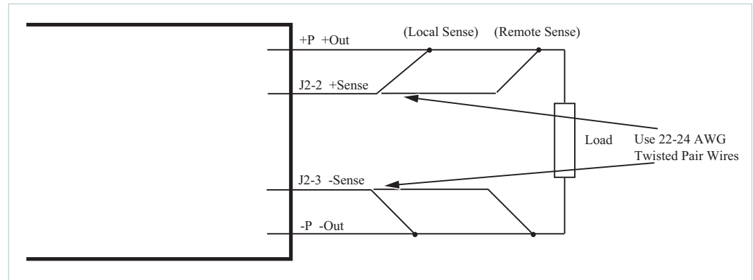
Figure 9. Sense Leads
