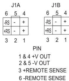
DualPAC Output Connector
