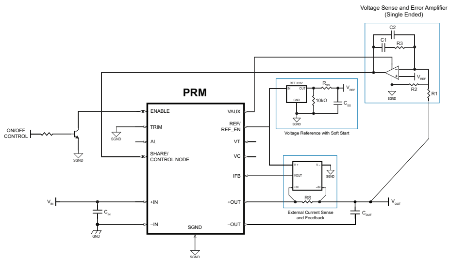
Remote Sense
