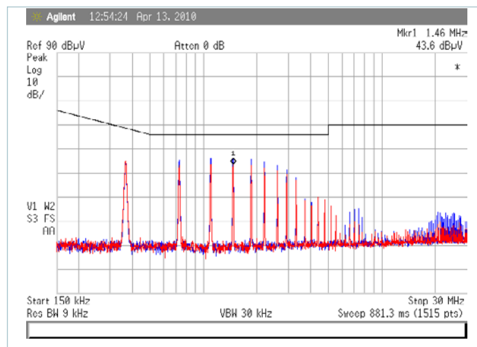
Figure 7 — V24B12C200BN using baseplate “Y” capacitors with a 136W load
