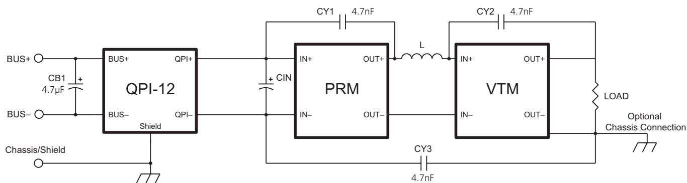
Figure 13 — PRM™/VTM™ in open-frame configuration with the output connected to the chassis/earth
