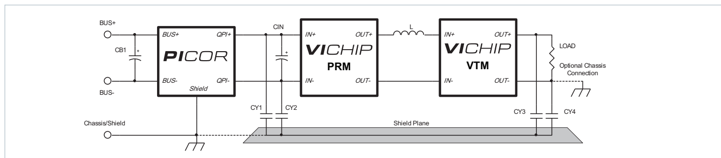
Figure 2 — Typical QPI-11 application schematic with Vicor's PRM and VTM modules in a baseplate configuration. [a]
