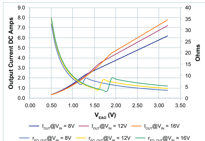
Figure 66 — r_{EQ\_OUT} vs. output current vs. V_{EAO} , V_{OUT} = 10V ; 8 – 16 V_{IN}
