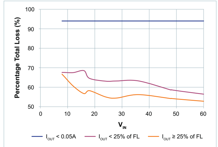
Figure 50 — V_{OUT} = 50V
