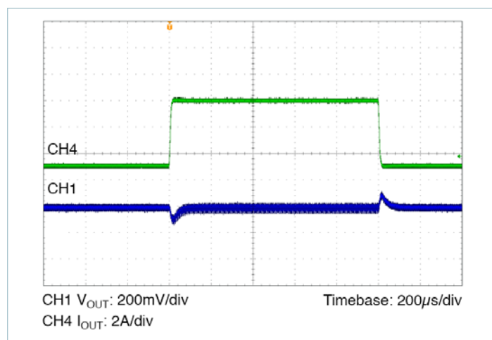
Figure 14 — Transient response: 5A to 10A, at 1A/μs. 48V IN to 3.3V OUT , C OUT = 6 x 100μF ceramic
