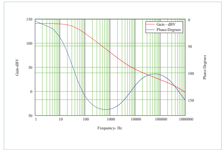
Figure 65 — G_{LGH\_EAO}(s) gain/phase plot R_{LGH} = 100k\Omega
