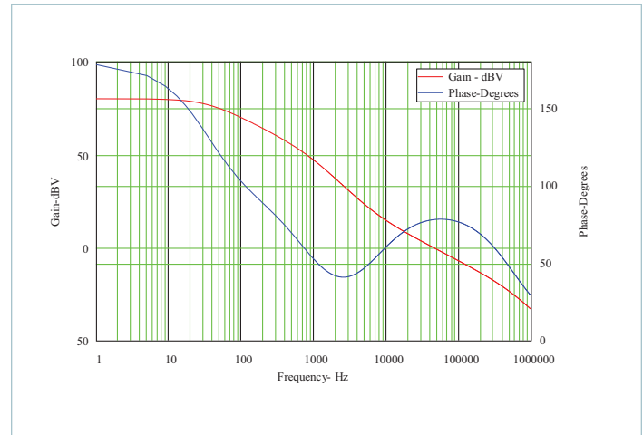
Figure 58 — PI354x-00 output-input gain/phase
