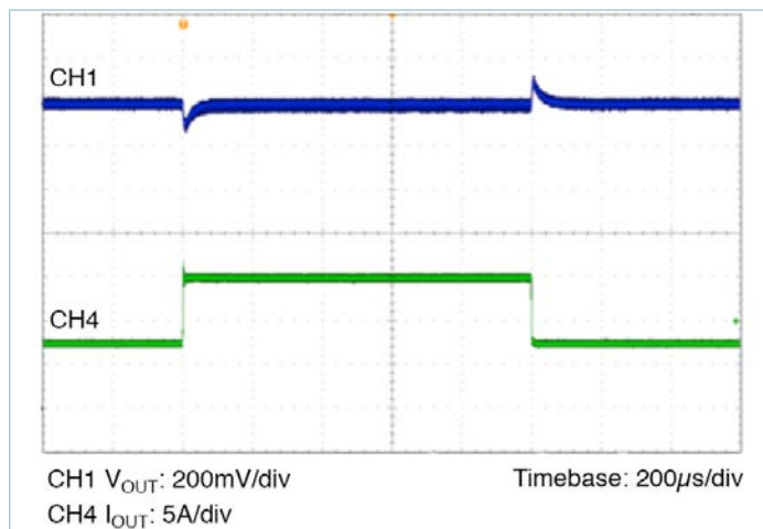
Figure 4 — Transient response 7.5A to 15A, at 5A/μs 24V IN to 3.3V OUT , C_{OUT} = 8 \times 100\mu F ceramic
