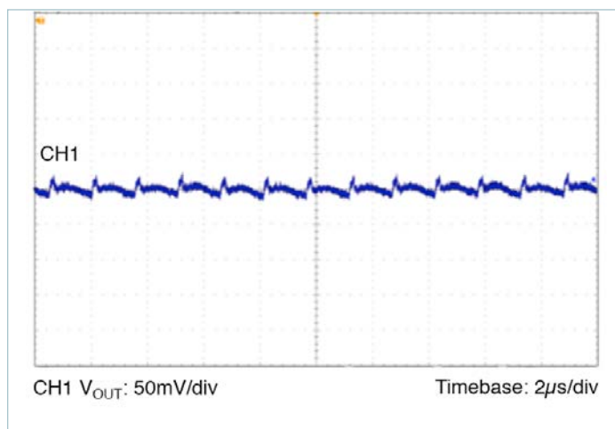
Figure 6 — Output ripple 24V IN , 3.3V OUT at 7.5A C_{OUT} = 8 \times 100\mu F ceramic
