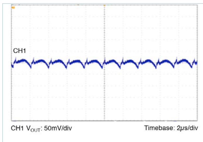
Figure 5 — Output ripple 24V IN , 3.3V OUT at 15A C_{OUT} = 8 \times 100\mu F ceramic
