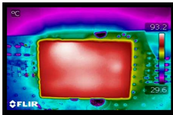
Figure 10 — Thermal image ( V_{IN} = 24V , I_{OUT} = 10A , CR, OLFM evaluation PCB)
