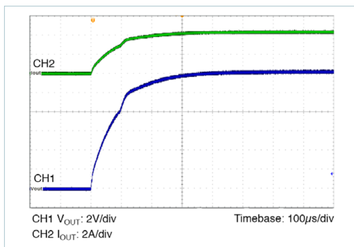
Figure 15 — Start-up C_{REF} = 0 ( V_{IN} = 18V , I_{OUT} = 4.2A , CR, C_{OUT} = 6 \times 2.2\mu F X7R ceramic)
