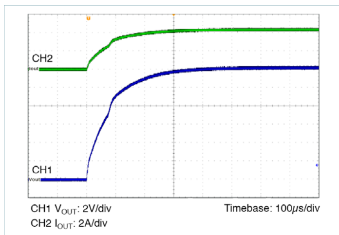
Figure 16 — Start-up C_{REF} = 0 ( V_{IN} = 24V , I_{OUT} = 4.2A , CR, C_{OUT} = 6 \times 2.2\mu F X7R ceramic)
