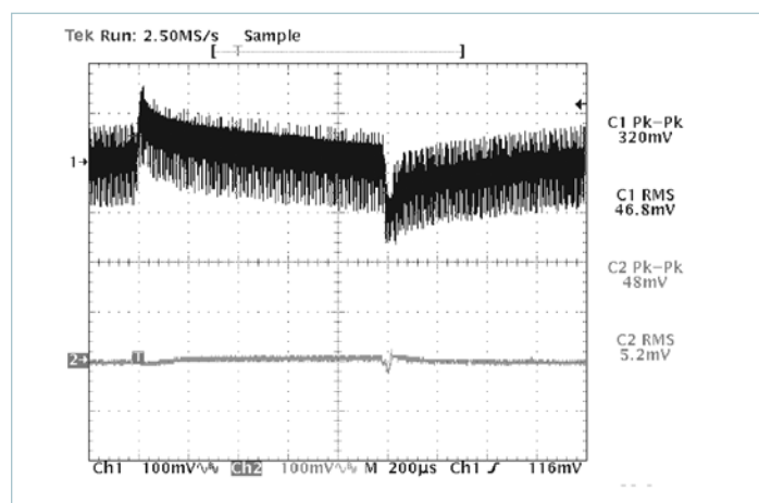
Figure 24 — V300B12C250B and μRAM; Input and output dynamic response C_{TRAN} = 820\mu\text{F} Electrolytic; 30% of load step of 6A (10A – 16A); R_{HR} = 80\text{k}\Omega (configured as in Figure 8 w/o Trim)
