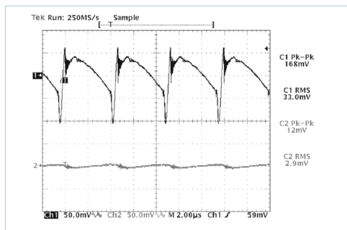
Figure 22 — V375B12C250B and μRAM; Input and output ripple @50% (10A) load CH1 = V_{IN} ; CH2 = V_{OUT} ; V_{IN} - V_{OUT} = 305\text{mV} ; R_{HR} = 80\text{k}\Omega (configured as in Figure 7 w/o Trim)
