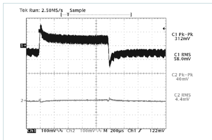
Figure 20 — V375A28C600B and μRAM; Input and output dynamic response no added C_{TRAN} ; 20% of 20A rating load step of 4A (10A – 14A); R_{HR} = 178\text{k}\Omega (configured as in Figure 7 w/o Trim)
