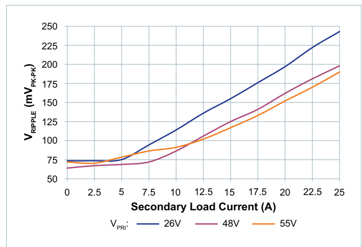
Figure 10 — V_{RIPPLE} vs. I_{SEC} : No external C_{SEC} . Board mounted module, scope setting: 20MHz analog BW
