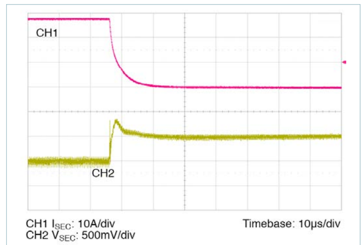
Figure 16 — Full load – 0A transient response: C_{PRI} = 100\mu\text{F} , no external C_{SEC}
