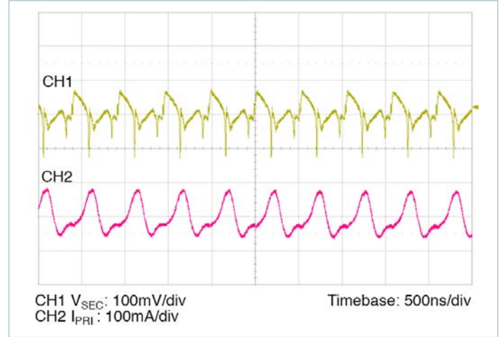
Figure 12 — Full load ripple, 100\mu\text{F} C_{PRI} ; No external C_{SEC} . Board-mounted module, scope setting: 20MHz analog BW
