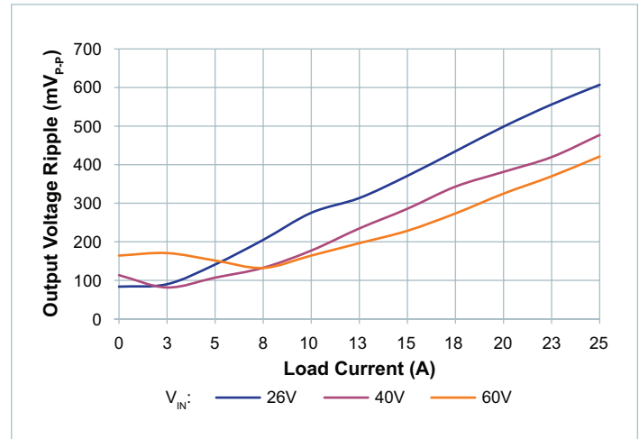
Figure 13 — Output voltage ripple ( V_{RIPPLE} ) vs. load ( I_{OUT} ); no external C_{OUT} .
