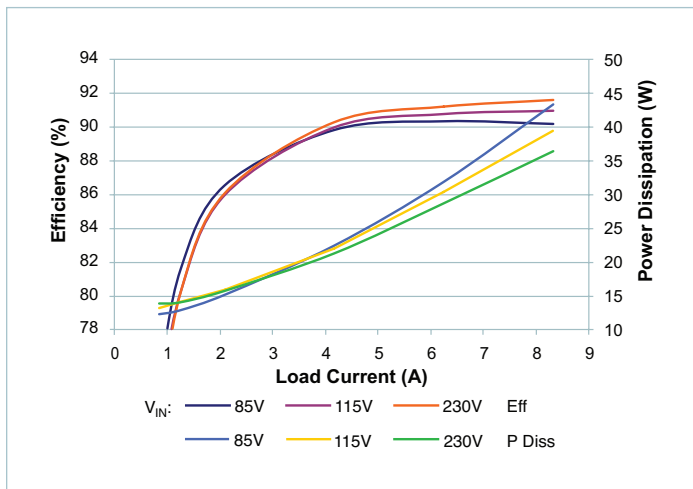
Figure 19 — V_{IN} to V_{OUT} efficiency and power dissipation vs. V_{IN} and I_{OUT} , T_{CASE} = 85^{\circ}\text{C}
