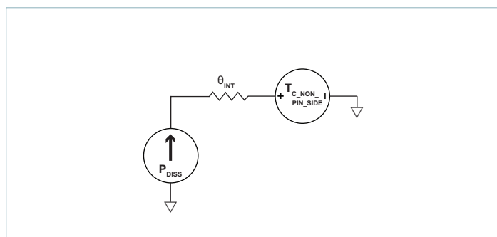
Figure 24 — Single-sided cooling thermal model
