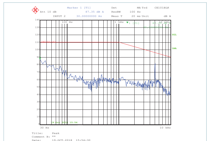
Figure 7 — Peak scan for the BLACK lead with C_{IN} = 11\mu F , R_{IN\_D} = 3.3\Omega , C_{OUT} = 2200\mu F , 100% load, V_{IN} = 160V
