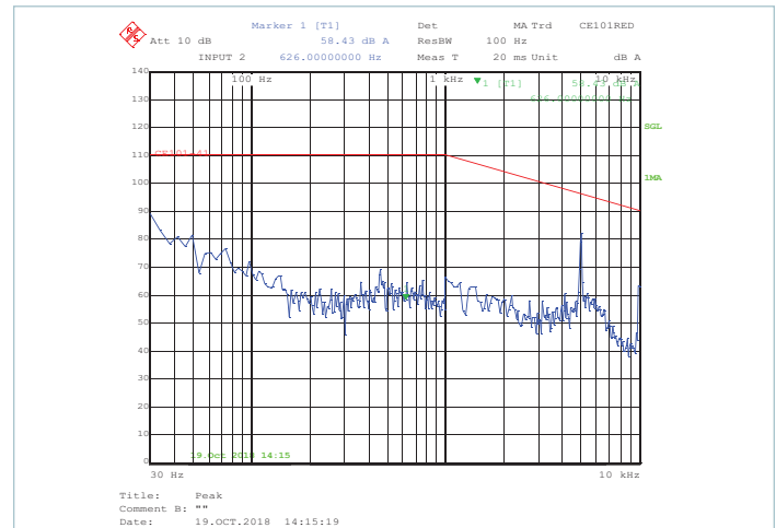
Figure 5 — Peak scan for the RED lead with C_{IN} = 11\mu F , R_{IN\_D} = 3.3\Omega , C_{OUT} = 2200\mu F , 100% load, V_{IN} = 160V
