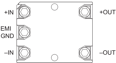
MFM1714 Filter – Chassis (Lug) Mount – Terminals Up
