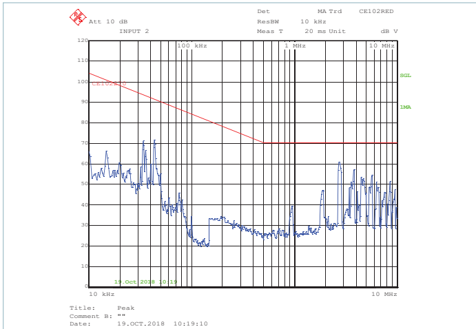
Figure 13 — Peak scan for the RED lead with C_{IN} = 11\mu F , R_{IN\_D} = 3.3\Omega , C_{OUT} = 2200\mu F , 0% load, V_{IN} = 160V
