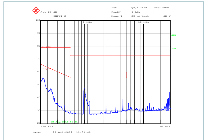
Figure 12 — Typical EMI spectrum, quasi-peak scan, 90% load, 230\text{V}_{IN} , C_{OUT} = 6,800\mu\text{F} ; test circuit – Figure 25
