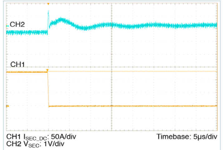
Figure 16 — 130 – 0A transient response:
