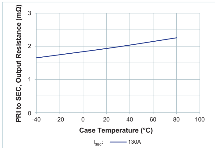
Figure 12 — R_{SEC} vs. temperature; nominal V_{PRI\_DC} I_{SEC\_DC} = 125\text{A} at T_{CASE} = 80^{\circ}\text{C}
