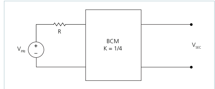
Figure 20 — K = 1/4 BCM with series primary resistor
