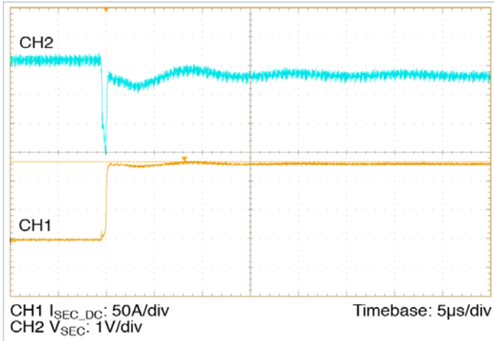
Figure 15 — 0 – 130A transient response:
