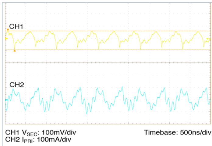
Figure 14 — Full-load secondary voltage and primary current ripple, 2700μF C_{PRI\_IN\_EXT} ; no external C_{SEC\_OUT\_EXT} . Board-mounted module, scope setting: 20MHz analog BW
