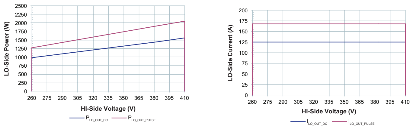
Figure 2 — Specified electrical operating area using rated R_{LO\_HOT}
