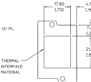
BOTTOM VIEW (HEATSINK AND THERMAL INTERFACE MATERIAL ONLY)
