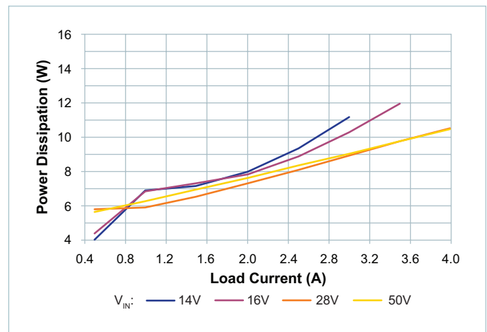
Figure 16 — Power dissipation at 100^\circ\text{C} case temperature, V_{OUT} = 50\text{V}
