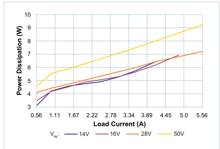
Figure 12 — Power dissipation at 100^\circ\text{C} case temperature, V_{OUT} = 26\text{V}
