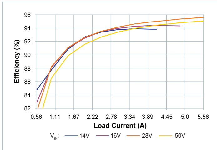
Figure 13 — Efficiency at 100^\circ\text{C} case temperature, V_{OUT} = 36\text{V}
