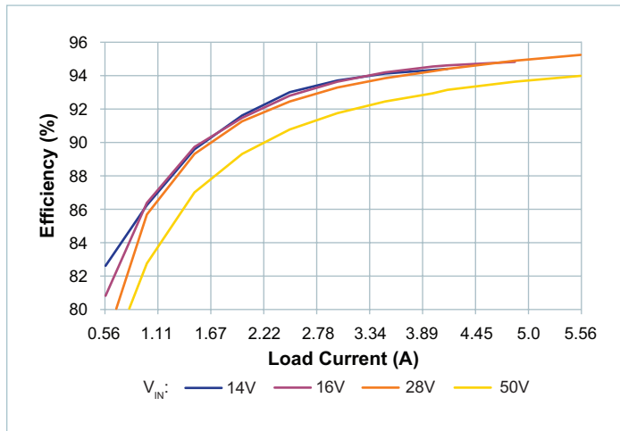
Figure 11 — Efficiency at 100^\circ\text{C} case temperature, V_{OUT} = 26\text{V}
