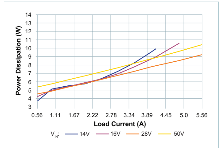
Figure 14 — Power dissipation at 100^\circ\text{C} case temperature, V_{OUT} = 36\text{V}
