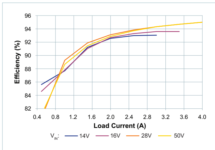
Figure 15 — Efficiency at 100^\circ\text{C} case temperature, V_{OUT} = 50\text{V}
