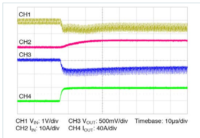
Figure 14 — 0 – 40A transient response: C_{IN} = 330\mu\text{F} , I_{IN} measured prior to C_{IN} , no external C_{OUT}
