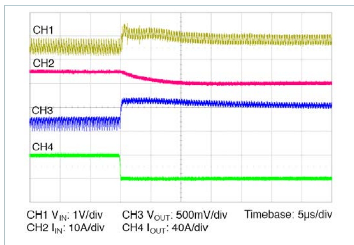
Figure 15 — 40 – 0A transient response: C_{IN} = 330\mu\text{F} , I_{IN} measured prior to C_{IN} , no external C_{OUT}
