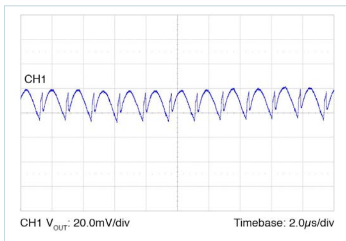
Figure 50 — Output voltage ripple: nominal line, nominal trim, 50% load, C_{OUT} = 6 \times 47\mu F ceramic, 20MHz BW
