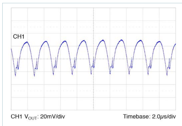
Figure 47 — Output voltage ripple: nominal line, nominal trim, 100% load, C_{OUT} = 6 \times 47\mu F ceramic, 20MHz BW
