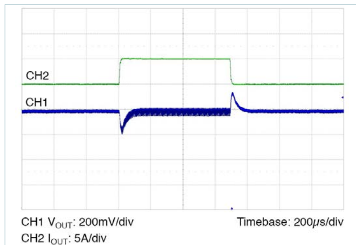
Figure 46 — Transient response: 50% to 100% load, at 1A/μs; nominal line, nominal trim, C_{OUT} = 6 \times 47\mu F ceramic
