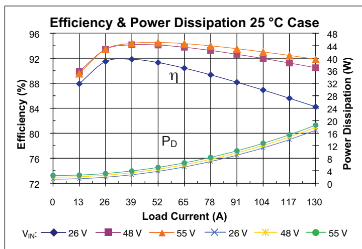
Figure 4 — Efficiency and power dissipation at 25\text{ }^{\circ}\text{C}
