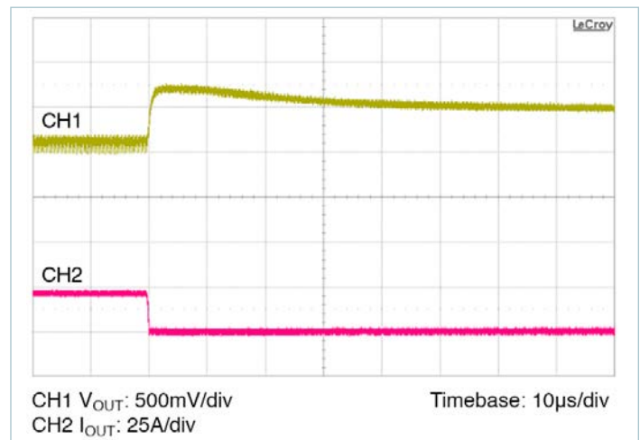
Figure 16 — Full load to 0A transient response: C_{IN} = 100\mu\text{F} , no external C_{OUT}
