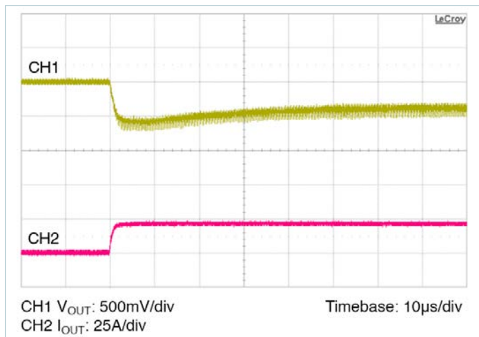
Figure 15 — 0A to Full load transient response: C_{IN} = 100\mu\text{F} , no external C_{OUT}
