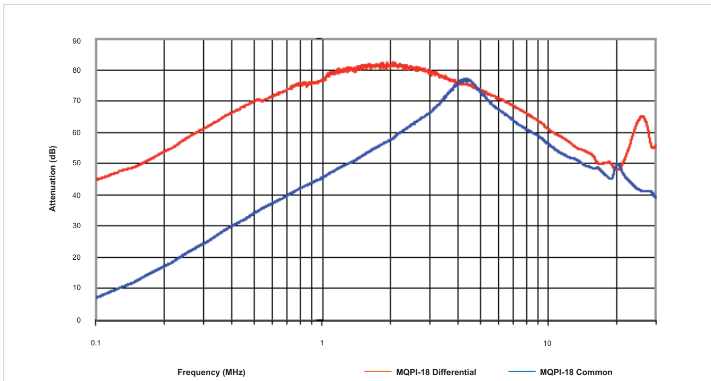
Figure 5 — Attenuation curves into a 50 Ω line impedance, bias from a 48 V bus
