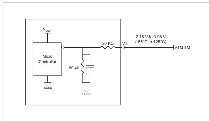
Figure 30 — VT Connections
