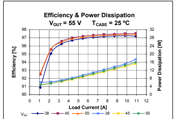
Figure 8 – Total efficiency and power dissipation vs. V_{IN} and I_{OUT} , V_{OUT}=55V , T_{CASE}=25^{\circ}C
