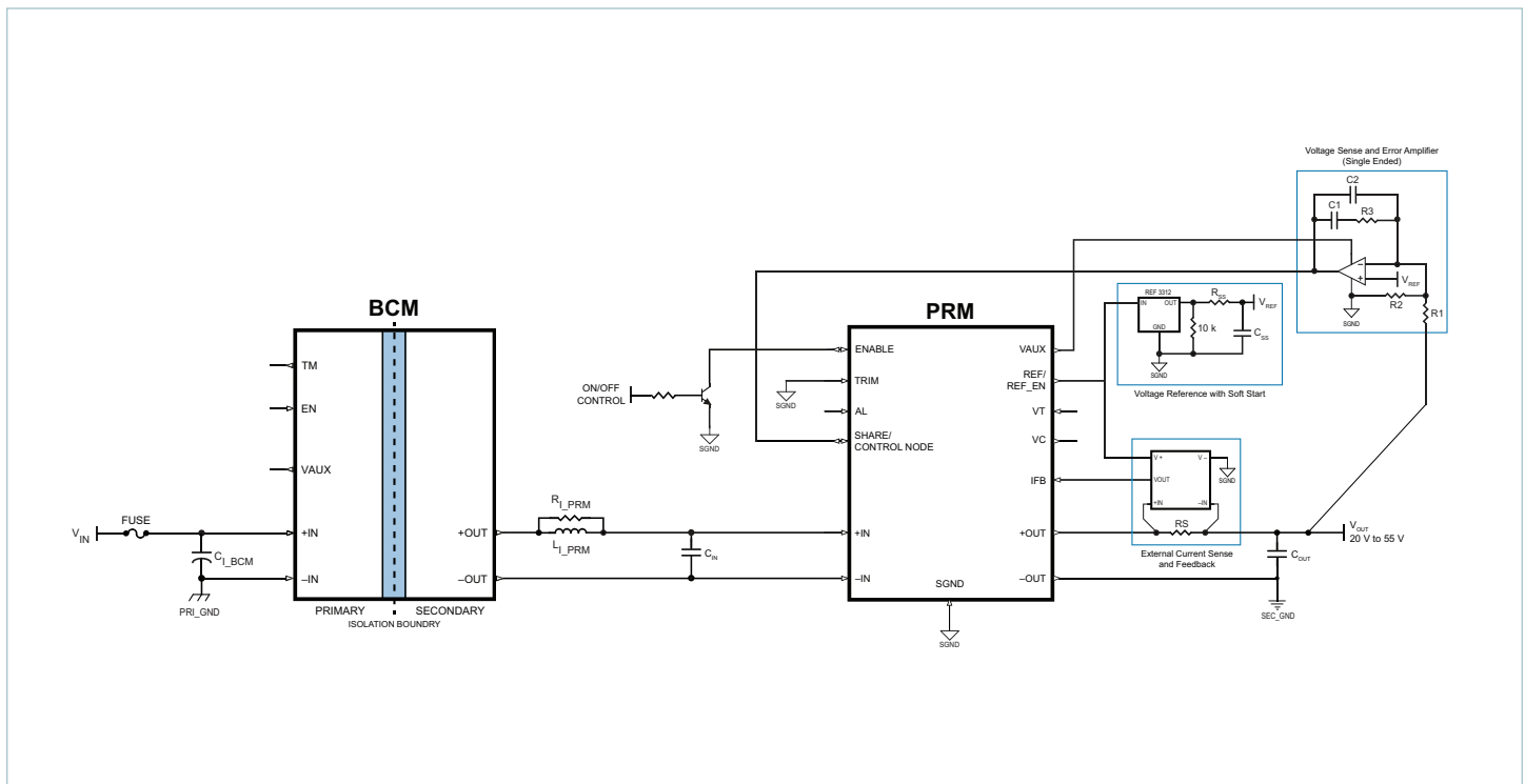
Typical Application: MBCM270 x 450M270A00 + MPRM48N x 480M500A00 Remote Sense Configuration
