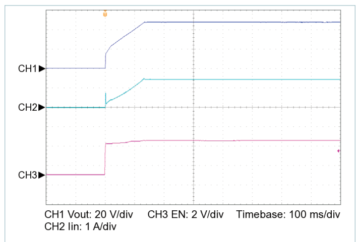
Figure 14 — Startup from EN, V_{IN} = 275\text{ V} , C_{OUT\_EXT} = 2000\text{ }\mu\text{F} , R_{LOAD} = 6.076\text{ }\Omega
