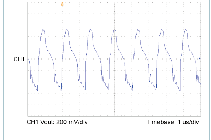
Figure 16 — Output voltage ripple, V_{IN} = 275\text{ V} , V_{OUT} = 48.0\text{ V} , C_{OUT\_EXT} = 200\text{ }\mu\text{F} , R_{LOAD} = 6.076\text{ }\Omega
