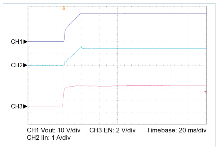
Figure 14 — Startup from EN, V_{IN} = 275\text{ V} , C_{OUT\_EXT} = 2000\text{ }\mu\text{F} , R_{LOAD} = 1.529\text{ }\Omega
