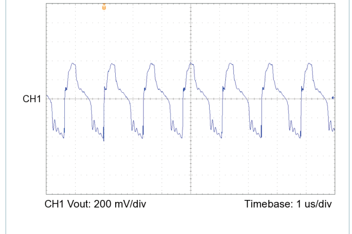
Figure 16 — Output voltage ripple, V_{IN} = 275\text{ V} , V_{OUT} = 24.0\text{ V} , C_{OUT\_EXT} = 200\text{ }\mu\text{F} , R_{LOAD} = 1.529\text{ }\Omega
