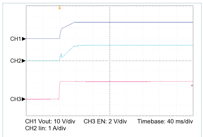
Figure 14 — Startup from EN, V_{IN} = 275\text{ V} , C_{OUT\_EXT} = 10000\text{ }\mu\text{F} , R_{LOAD} = 0.600\text{ }\Omega
