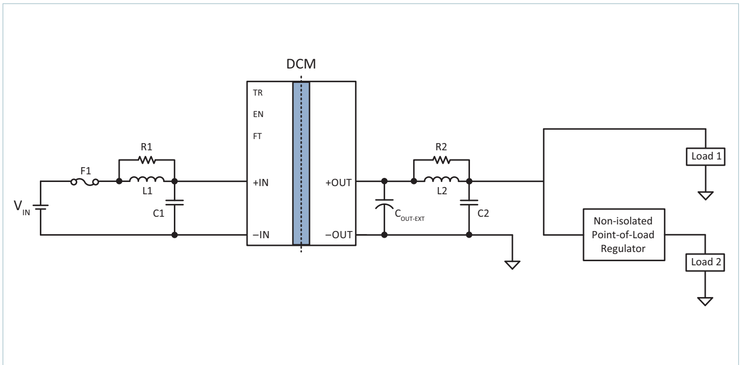
Typical Application 1: Single DCM4623xD2N13C8y7z, to a non-isolated regulator, and direct to load
