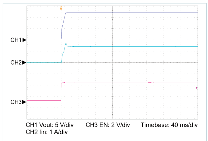
Figure 14 — Startup from EN, V_{IN} = 275\text{ V} , C_{OUT\_EXT} = 10000\text{ }\mu\text{F} , R_{LOAD} = 0.383\text{ }\Omega
