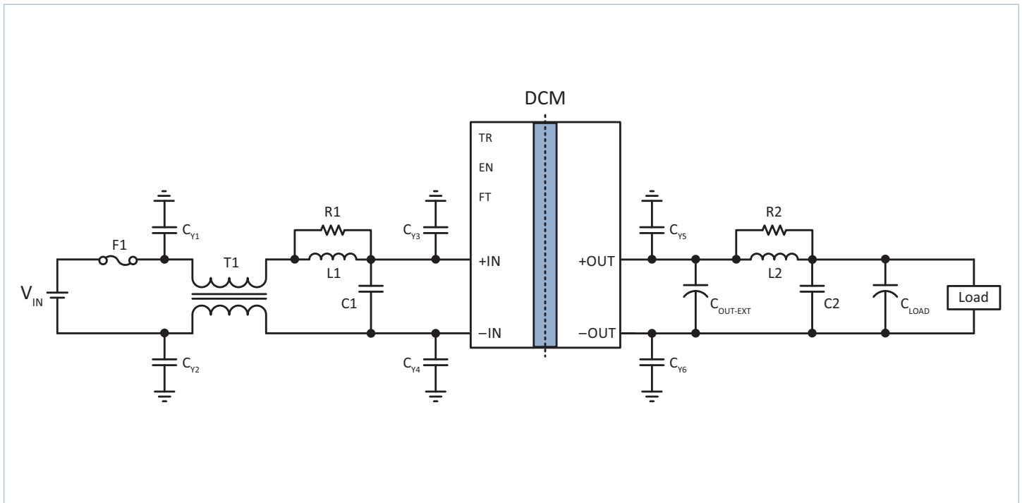
Typical Application 2: Single DCM4623xD2N13C8y7z with common- and differential-mode input filters
