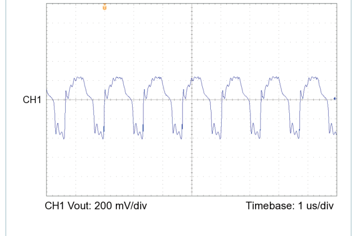
Figure 16 — Output voltage ripple, V_{IN} = 275\text{ V} , V_{OUT} = 12.0\text{ V} , C_{OUT\_EXT} = 1000\text{ }\mu\text{F} , R_{LOAD} = 0.383\text{ }\Omega
