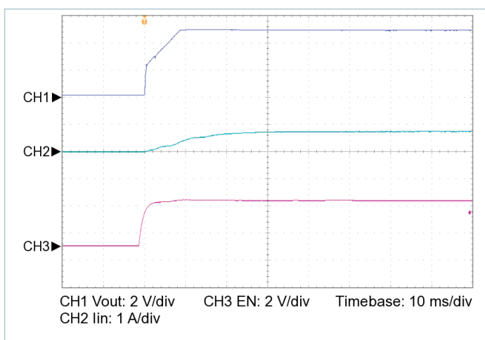
Figure 14 — Startup from EN, V_{IN} = 275\text{ V} , C_{OUT\_EXT} = 10000\text{ }\mu\text{F} , R_{LOAD} = 0.132\text{ }\Omega
