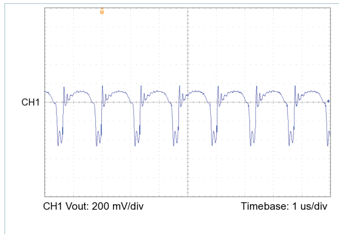
Figure 16 — Output voltage ripple, V_{IN} = 275\text{ V} , V_{OUT} = 5.0\text{ V} , C_{OUT\_EXT} = 1000\text{ }\mu\text{F} , R_{LOAD} = 0.132\text{ }\Omega
