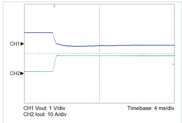
Figure 8 — 10% to 100% load transient response, V_{IN} = 270\text{ V} , nominal trim, C_{OUT\_EXT} = 200\text{ }\mu\text{F}
