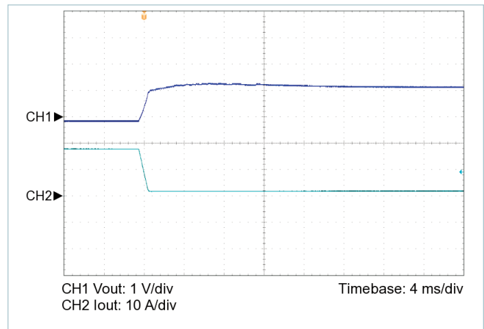
Figure 7 — 100% to 10% load transient response, V_{IN} = 270\text{ V} , nominal trim, C_{OUT\_EXT} = 200\text{ }\mu\text{F}
