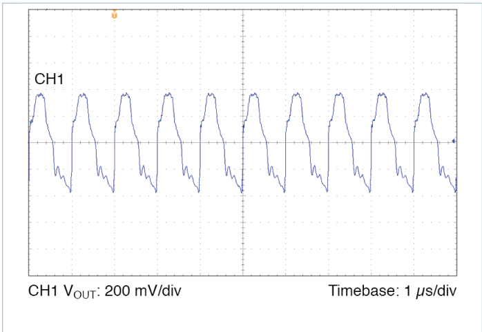
Figure 19 — Output voltage ripple, V_{IN} = 270\text{ V} , V_{OUT} = 24.0\text{ V} , C_{OUT\_EXT} = 220\text{ }\mu\text{F} , R_{LOAD} = 1.152\text{ }\Omega
