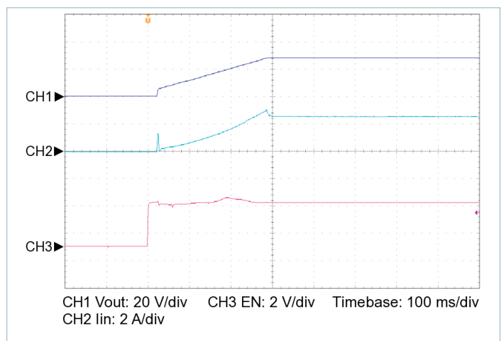
Figure 14 — Startup from EN, V_{IN} = 100\text{ V} , C_{OUT\_EXT} = 20000\text{ }\mu\text{F} , R_{LOAD} = 3.256\text{ }\Omega
