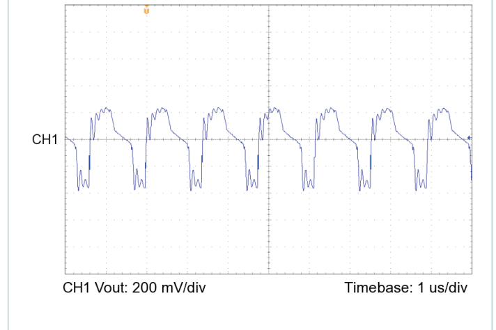
Figure 16 — Output voltage ripple, V_{IN} = 100\text{ V} , V_{OUT} = 28.0\text{ V} , C_{OUT\_EXT} = 1000\text{ }\mu\text{F} , R_{LOAD} = 3.256\text{ }\Omega
