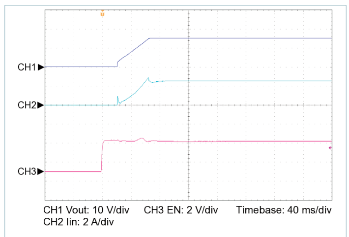
Figure 14 — Startup from EN, V_{IN} = 100\text{ V} , C_{OUT\_EXT} = 20000\text{ }\mu\text{F} , R_{LOAD} = 0.938\text{ }\Omega
